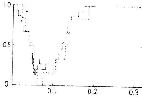
図 1. Ambiguity vs. \bar{D}_C / \bar{D}_F
