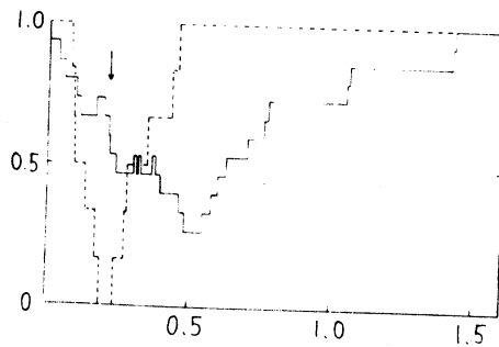
図 3. Ambiguity vs. \bar{D}_C / \bar{D}_\beta
