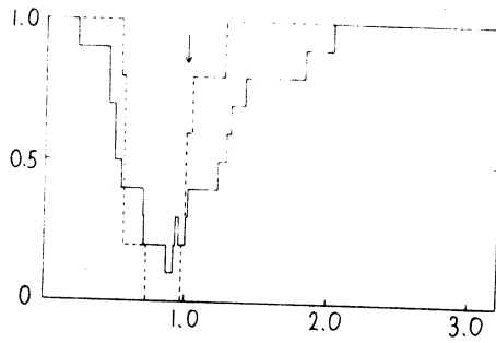
図 2. Ambiguity vs. \bar{D}_{H\alpha} / \bar{D}_{H\beta}
